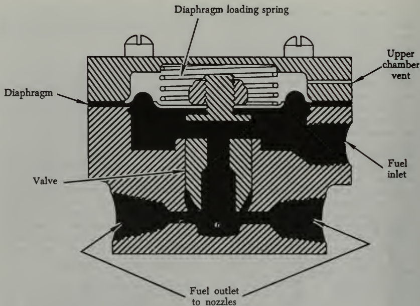
FIGURE 3-38. Fuel manifold valve assembly.
